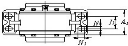
N1 KOYO V532 One-piece type
